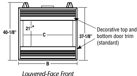
Louvered-Face Front
