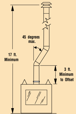
Typical Installation
