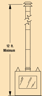
Typical Installation
