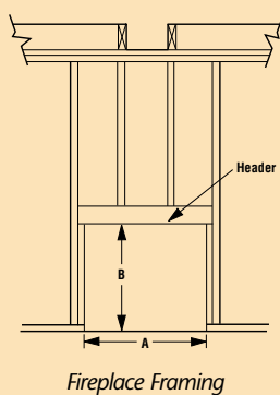
Fireplace Framing
