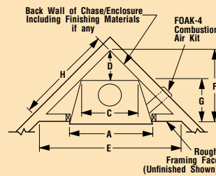
Corner Installation
